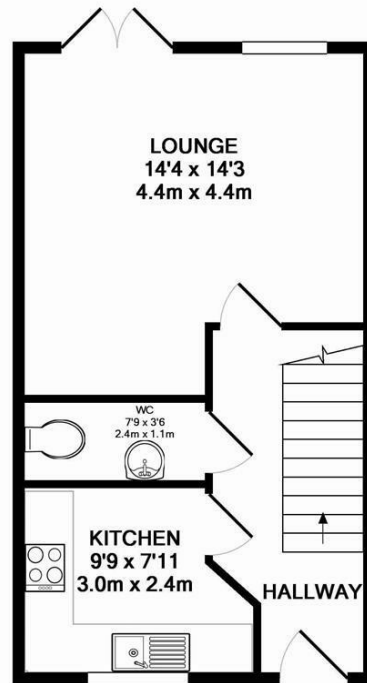
GROUND FLOOR APPROX. FLOOR AREA 367 SQ.FT. (34.1 SQ.M.)
